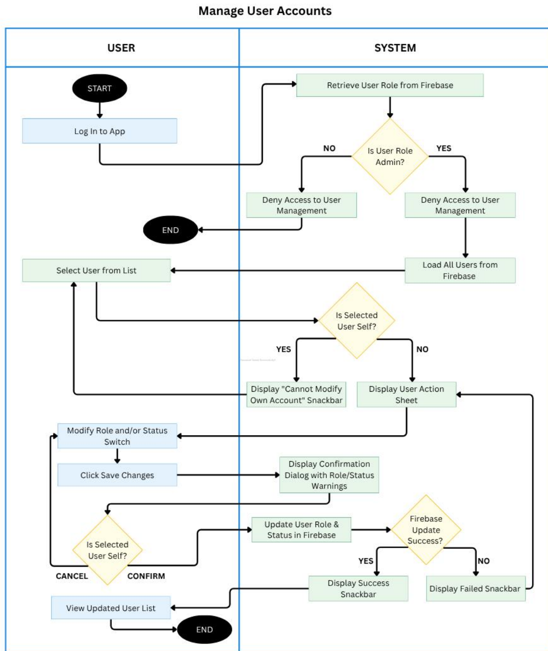
Figure 3.14. Activity Diagram for Manage User Accounts
